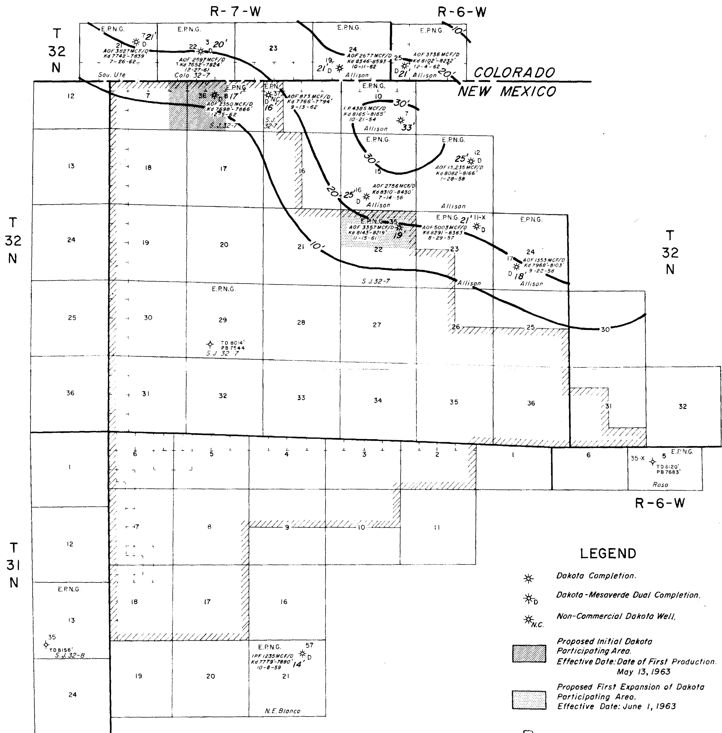
EXHIBIT "C" FIGURE NO. 2 SAN JUAN 32-7 UNIT SAN JUAN COUNTY, NEW MEXICO ISOPACH MAP NET RESERVOIR SANDS - DAKOTA PRODUCING INTERVAL CONTOUR INTERVAL = 10 FEET
