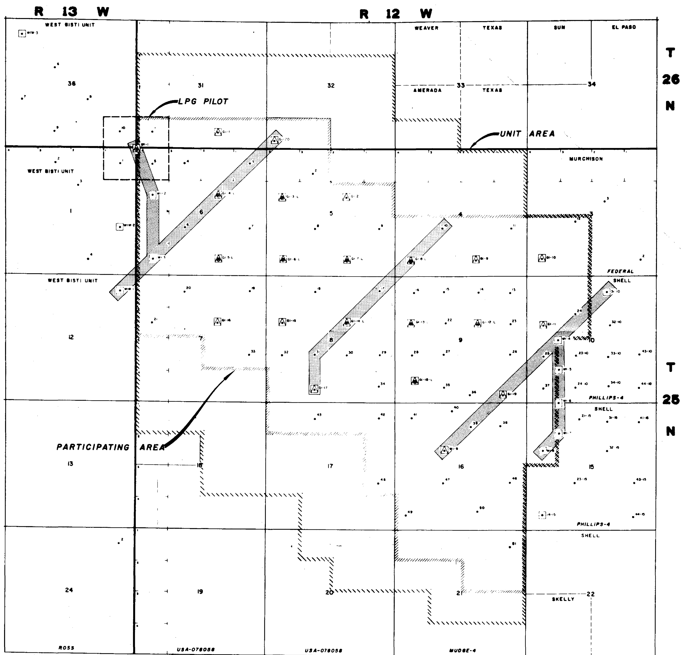
PROPOSED INJECTION PATTERN SEPT 1963
