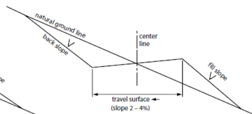
Typical Insloped Section
