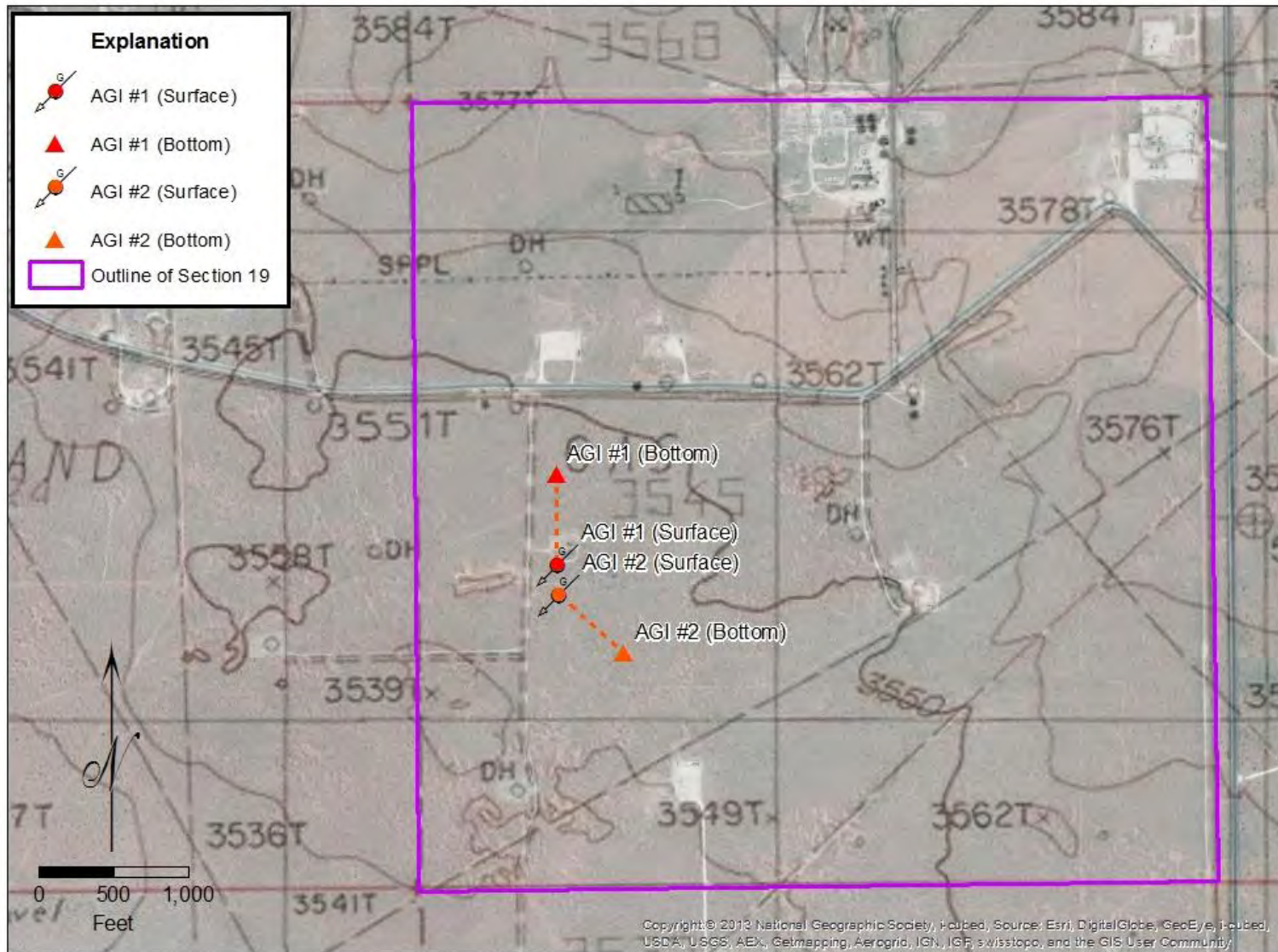
Figure 1a: Surface and Bottom Hole Locations of Zia AGI #1 and AGI #2
