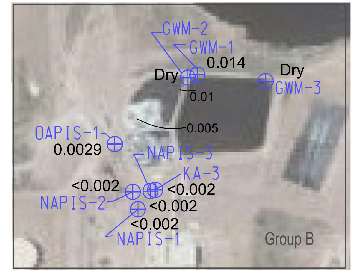
Total Xylenes (11/11/13)
