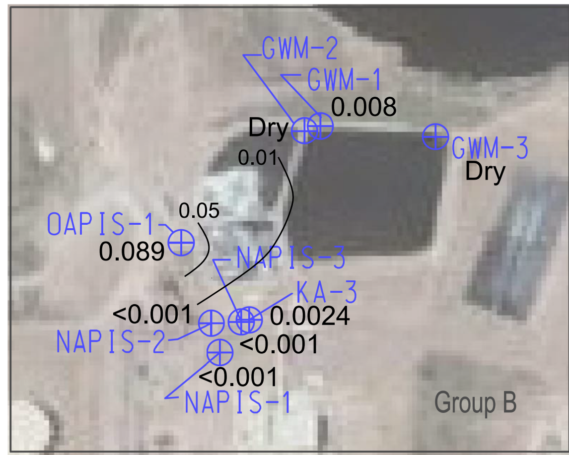
Benzene (11/11/13)
