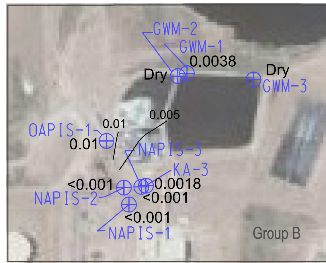
Ethyl Benzene (11/11/13)
