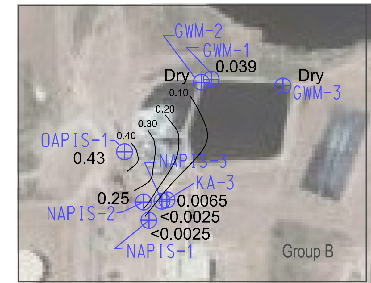
MTBE (11/11/13)
