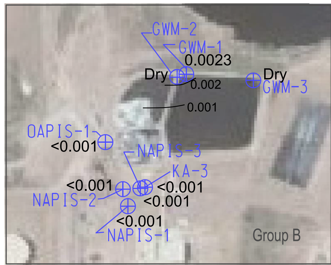
Toluene (11/11/13)
