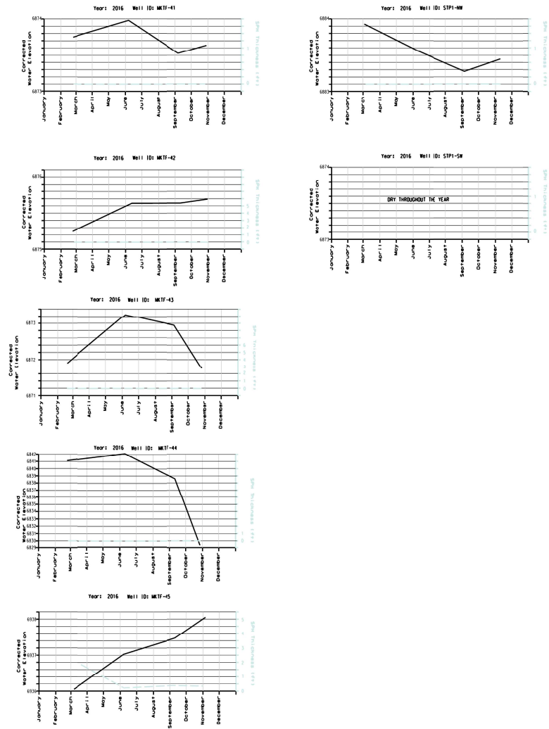
Figure 11C GROUNDWATER ELEVATION VS TIME WESTERN REFINING - GALLUP REFINERY
