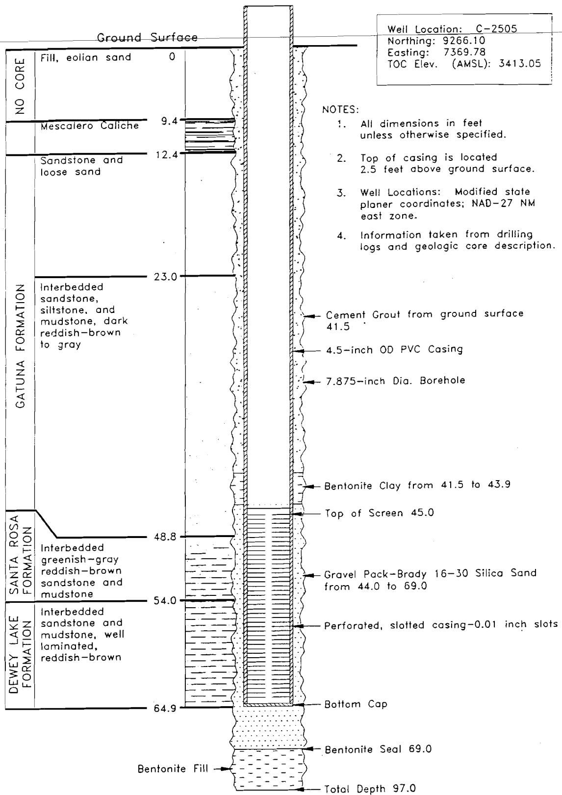
Figure 2.1. C-2505 well completion diagram.
