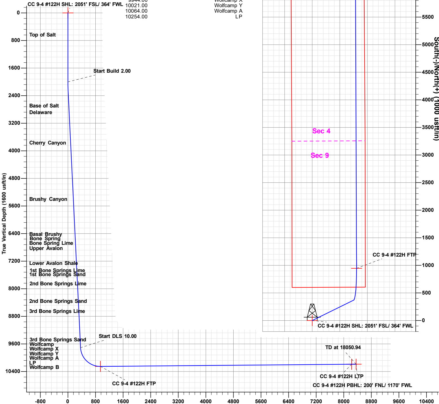
Vertical Section at 359.77° (1600 usft/in)
