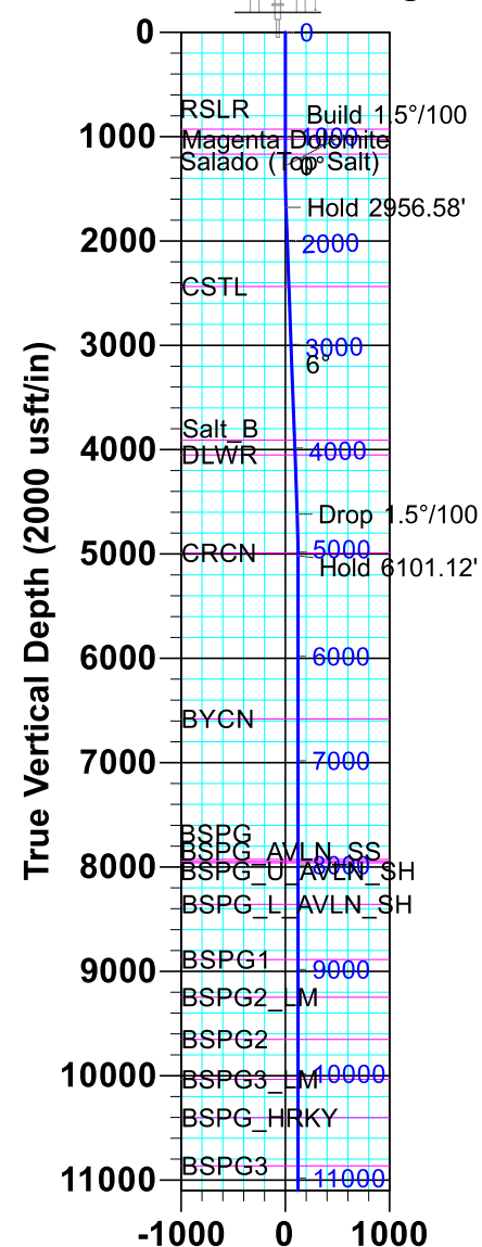
Vertical Section at 180.05° (2000 usft/in)
