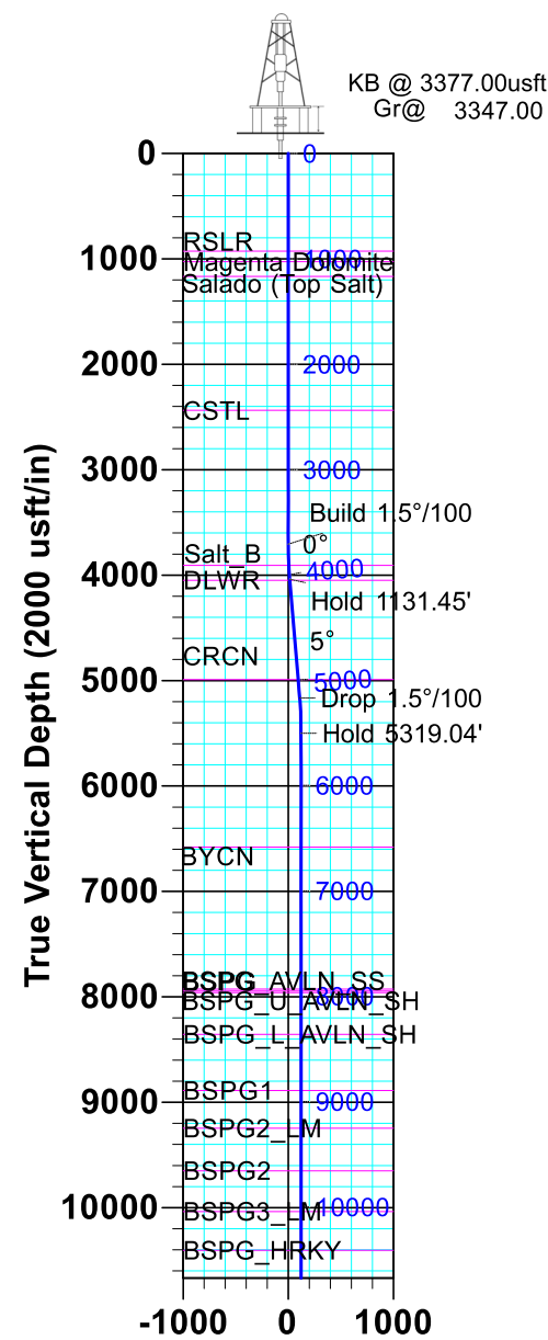
Vertical Section at 180.05° (2000 usft/in)
