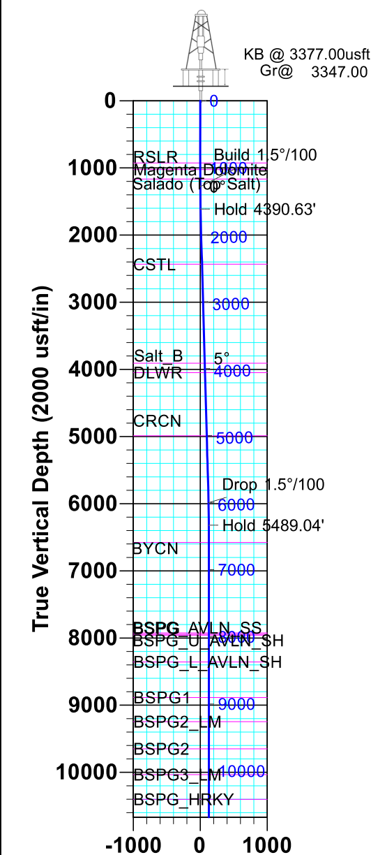
Vertical Section at 180.05° (2000 usft/in)
