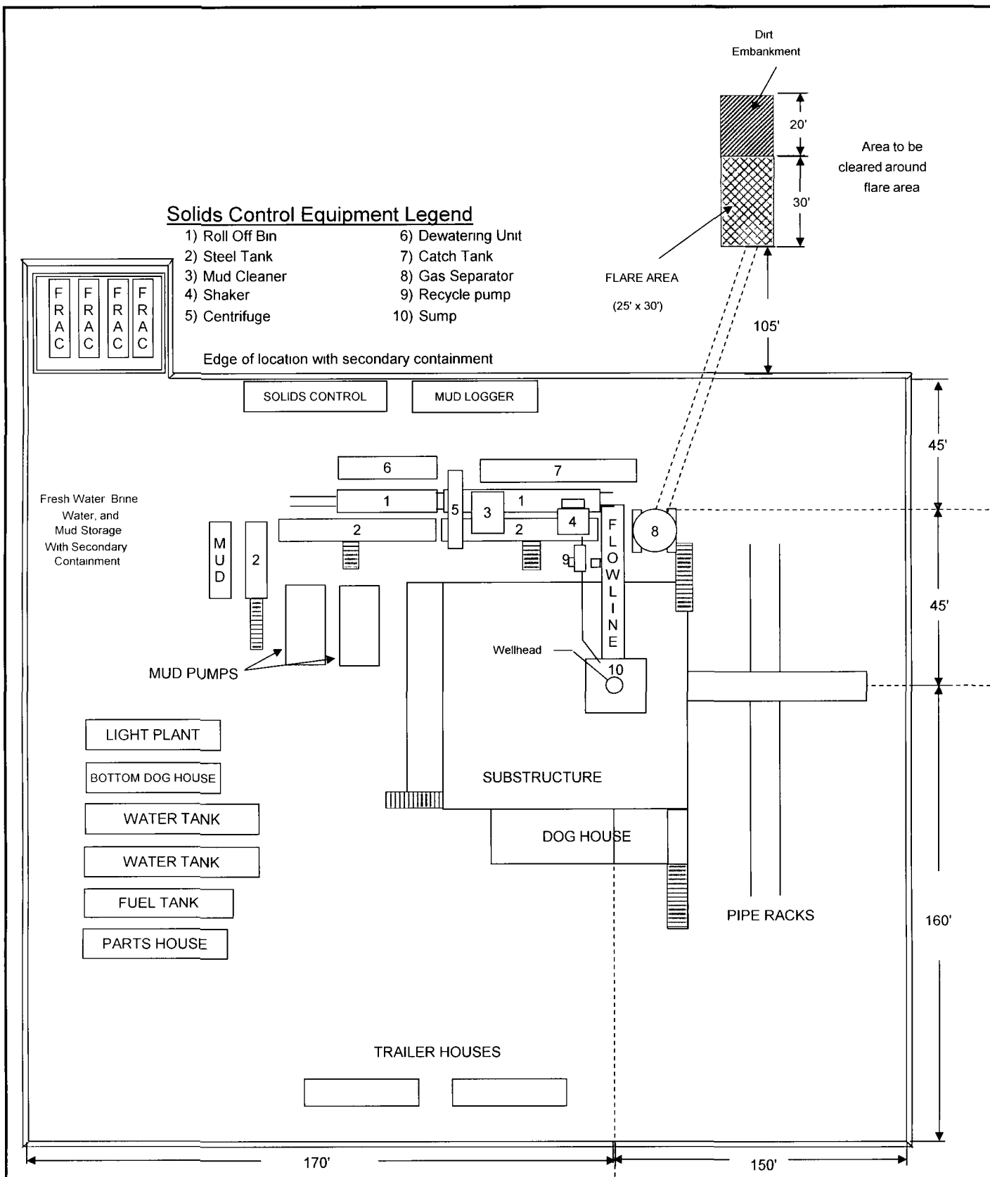
POKER LAKE UNIT 312H TYPICAL RIG LAYOUT SCHEMATIC INCLUSIVE OF CLOSED-LOOP DESIGN PLAN
