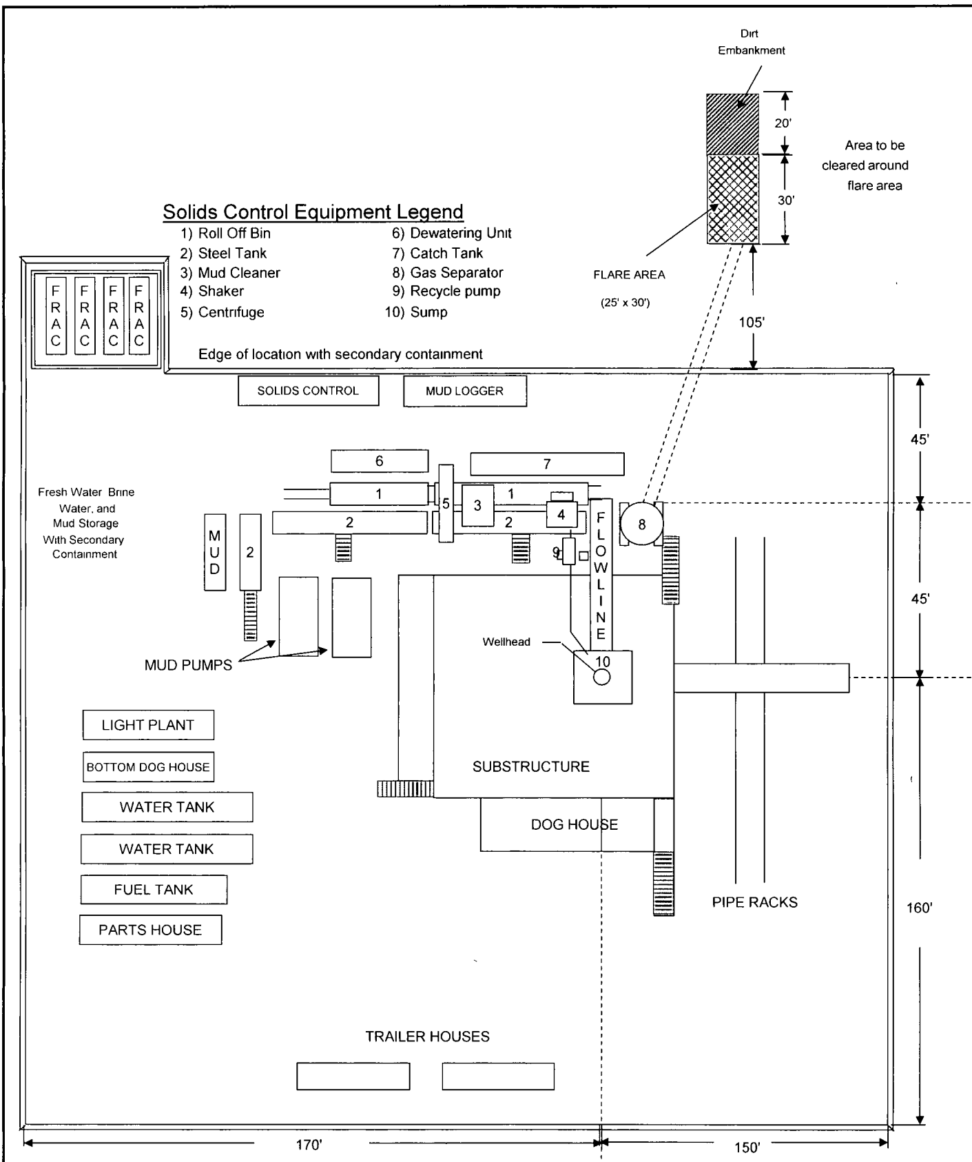
POKER LAKE UNIT 337H TYPICAL RIG LAYOUT SCHEMATIC INCLUSIVE OF CLOSED-LOOP DESIGN PLAN
