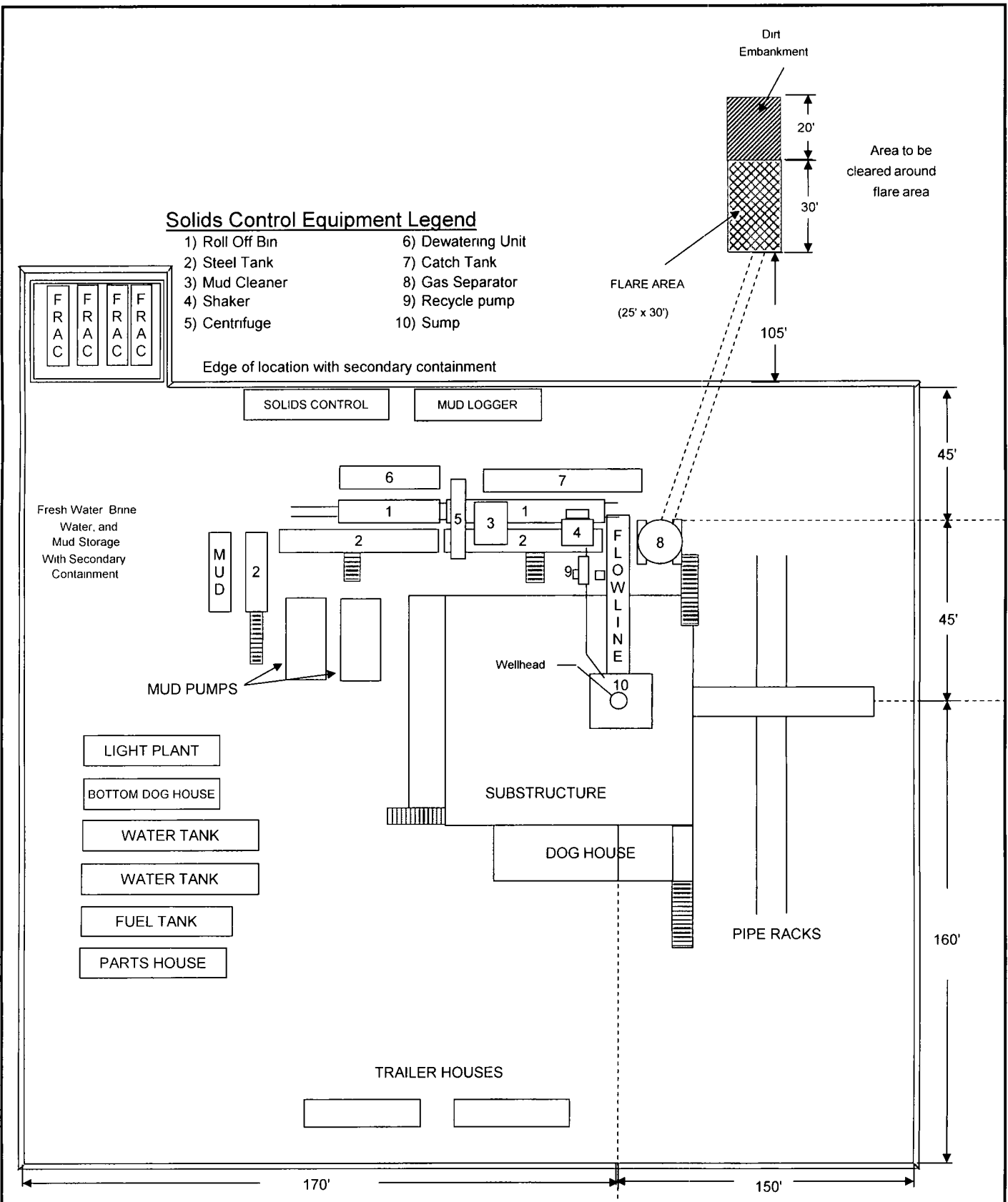
POKER LAKE UNIT 318H TYPICAL RIG LAYOUT SCHEMATIC INCLUSIVE OF CLOSED-LOOP DESIGN PLAN
