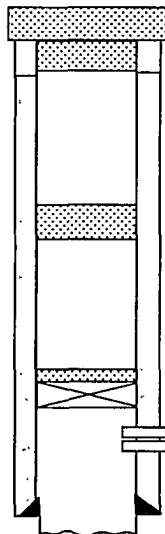
Plug 2: 100' plug fr/650'-750'.
