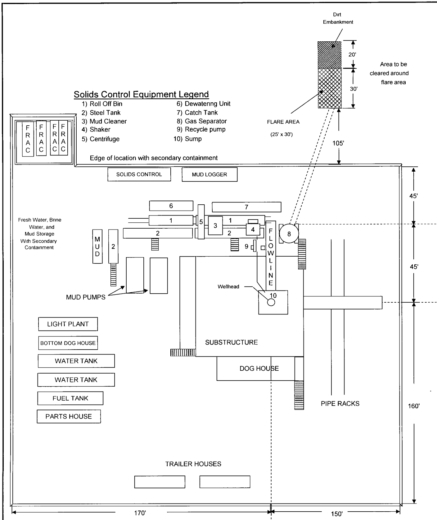
POKER LAKE UNIT 370H TYPICAL RIG LAYOUT SCHEMATIC INCLUSIVE OF CLOSED-LOOP DESIGN PLAN
