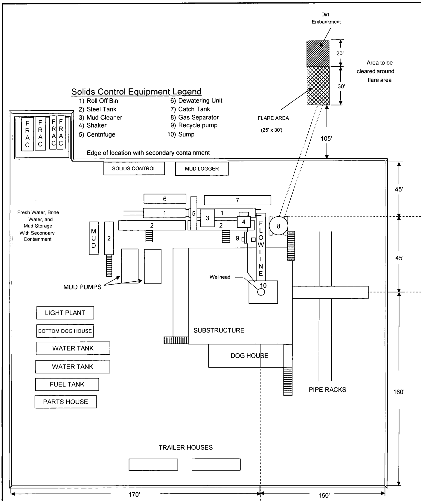
POKER LAKE UNIT 423H TYPICAL RIG LAYOUT SCHEMATIC INCLUSIVE OF CLOSED-LOOP DESIGN PLAN
