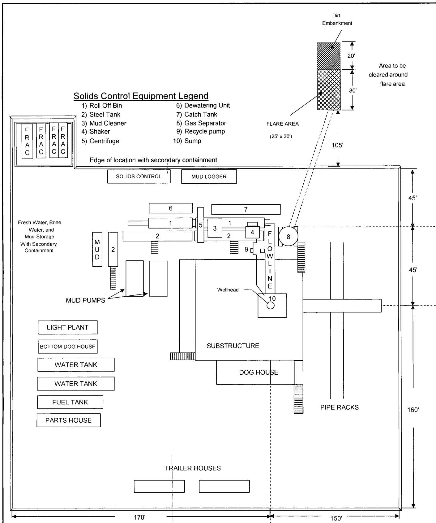
POKER LAKE UNIT 410H TYPICAL RIG LAYOUT SCHEMATIC INCLUSIVE OF CLOSED-LOOP DESIGN PLAN
