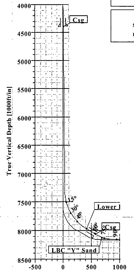
Vertical Section at 132.80° [1000ft/in]
