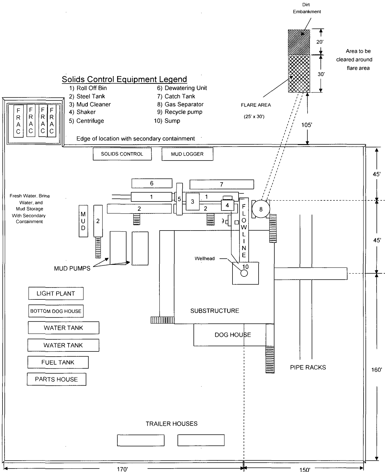
NASH DRAW "8" FEDERAL 1 SWD TYPICAL RIG LAYOUT SCHEMATIC INCLUSIVE OF CLOSED-LOOP DESIGN PLAN
