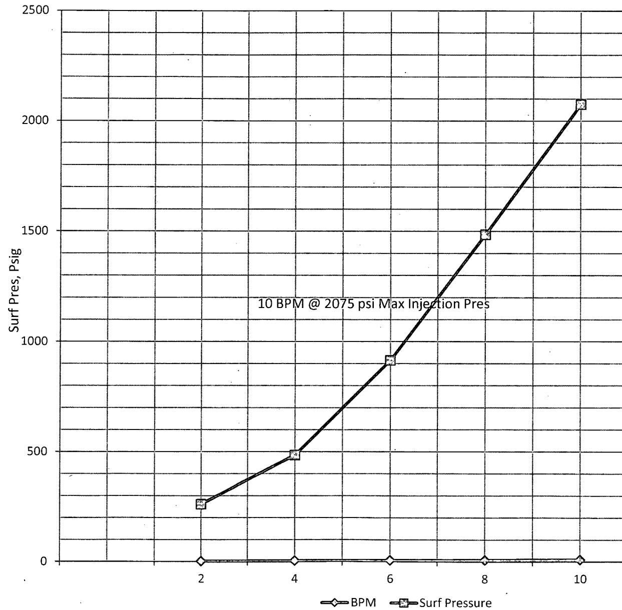
Apache State SWD #3 - Step-Rate Injectivity - Surface Pressure (4 1/2" Tubing)
