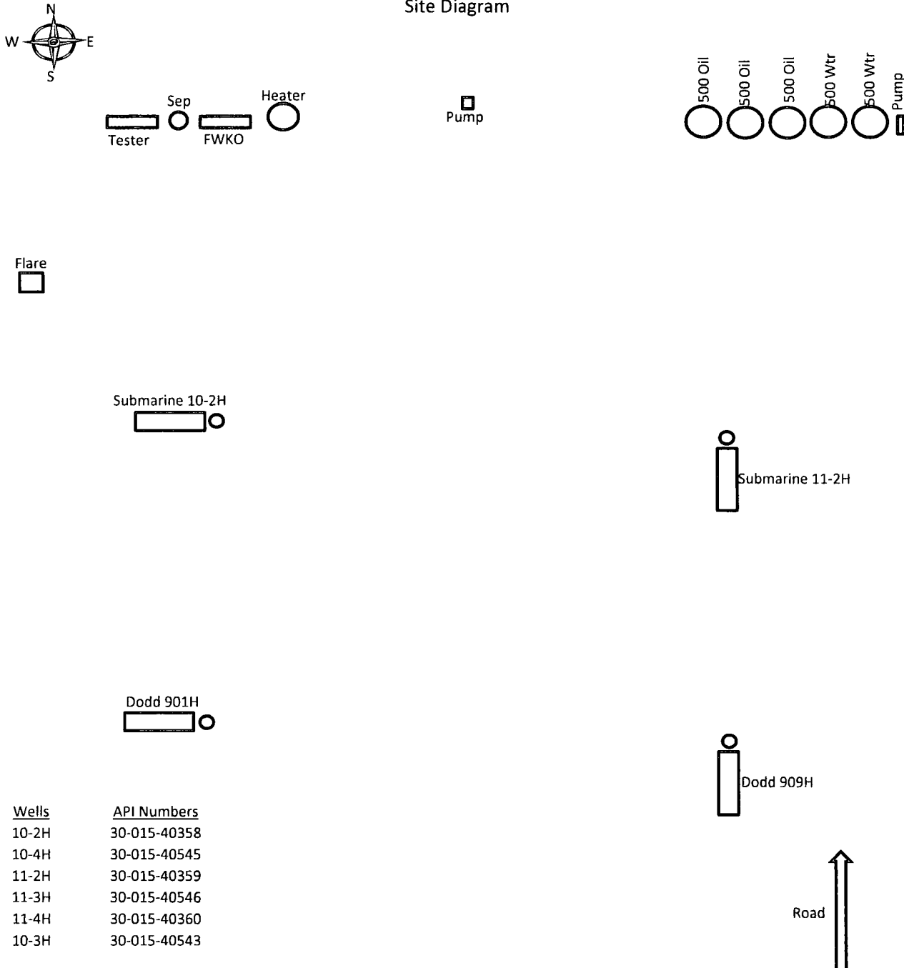
Site Diagram
