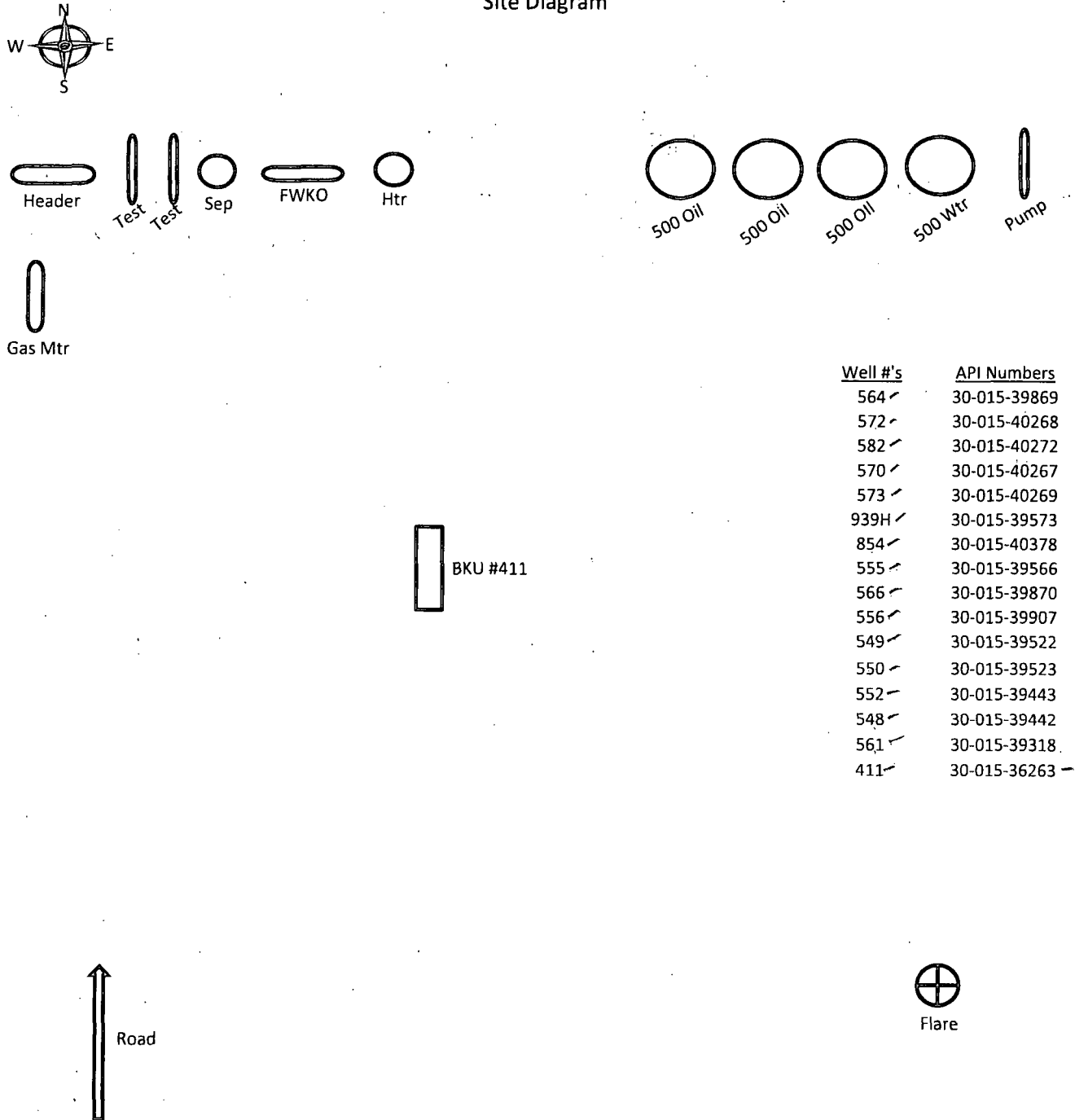
Site Diagram
