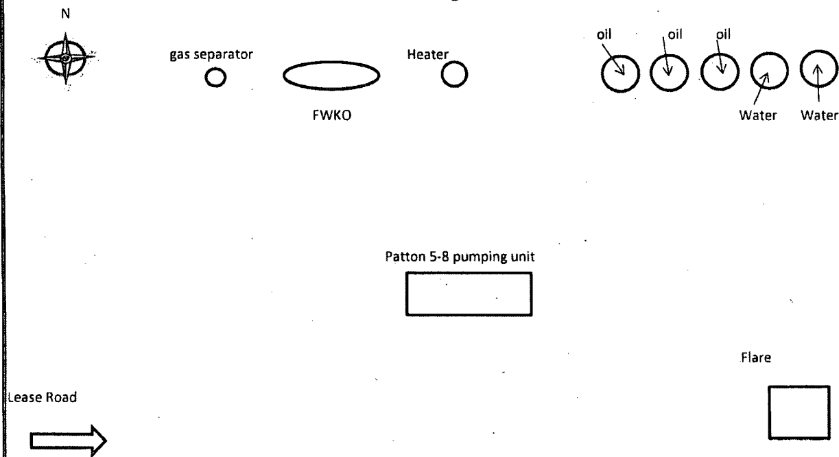
Site Diagram
