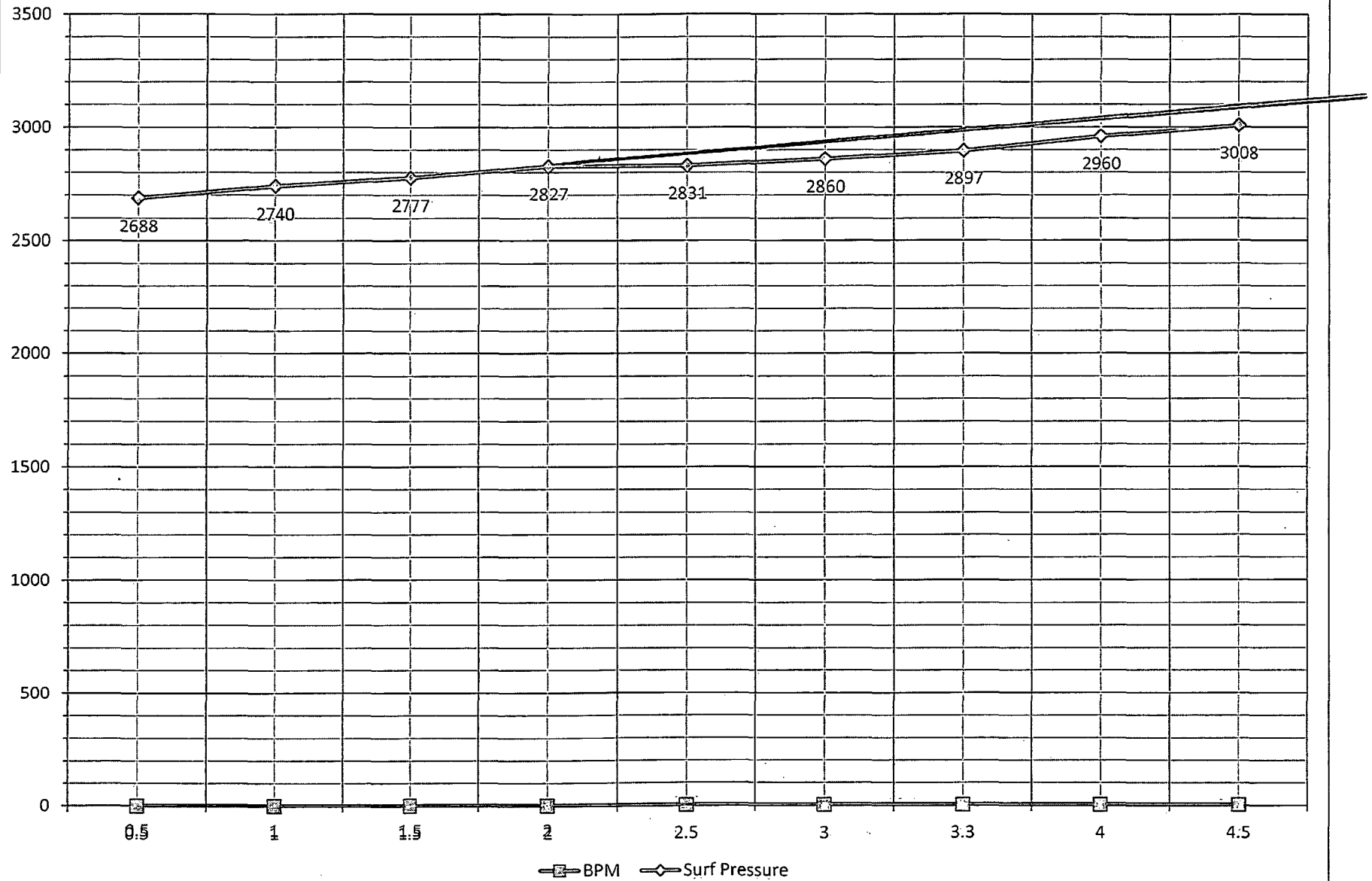
Barnsdall #1 - Step-Rate Injectivity - Surface Pressure
