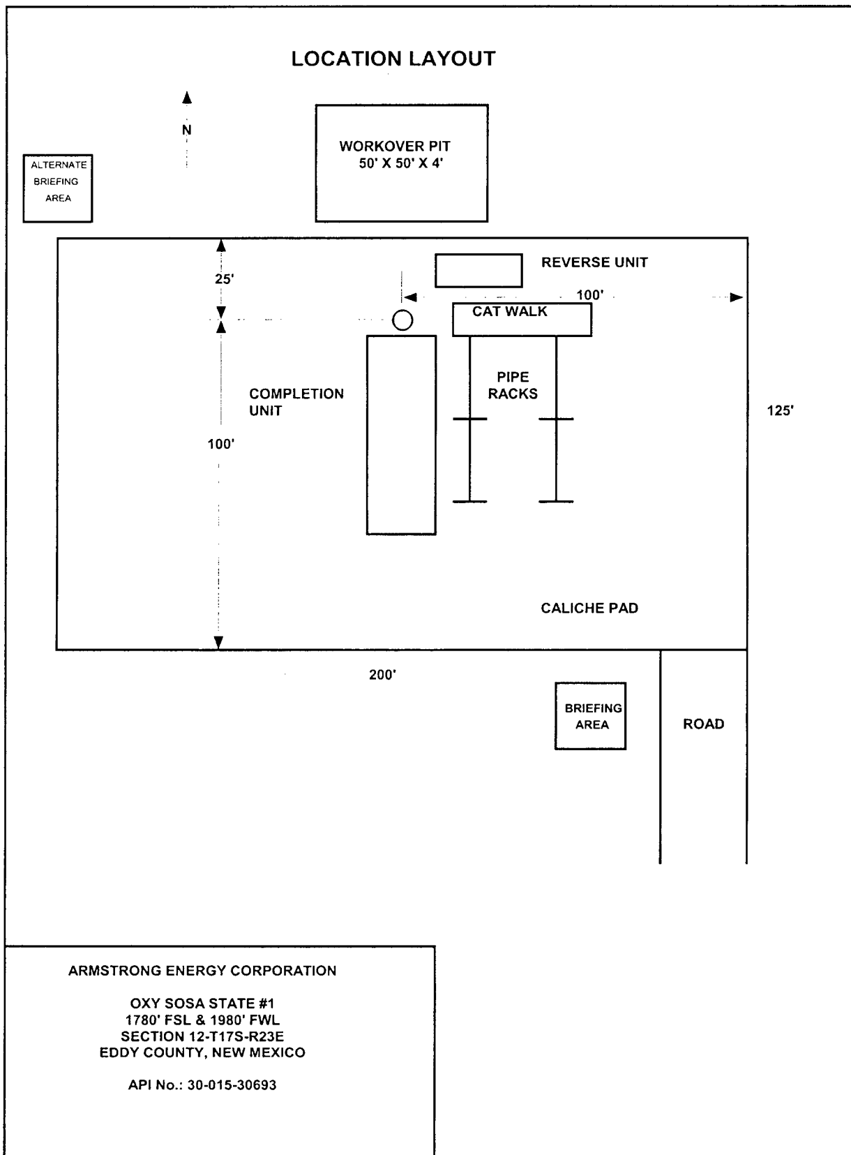
Location Layout
