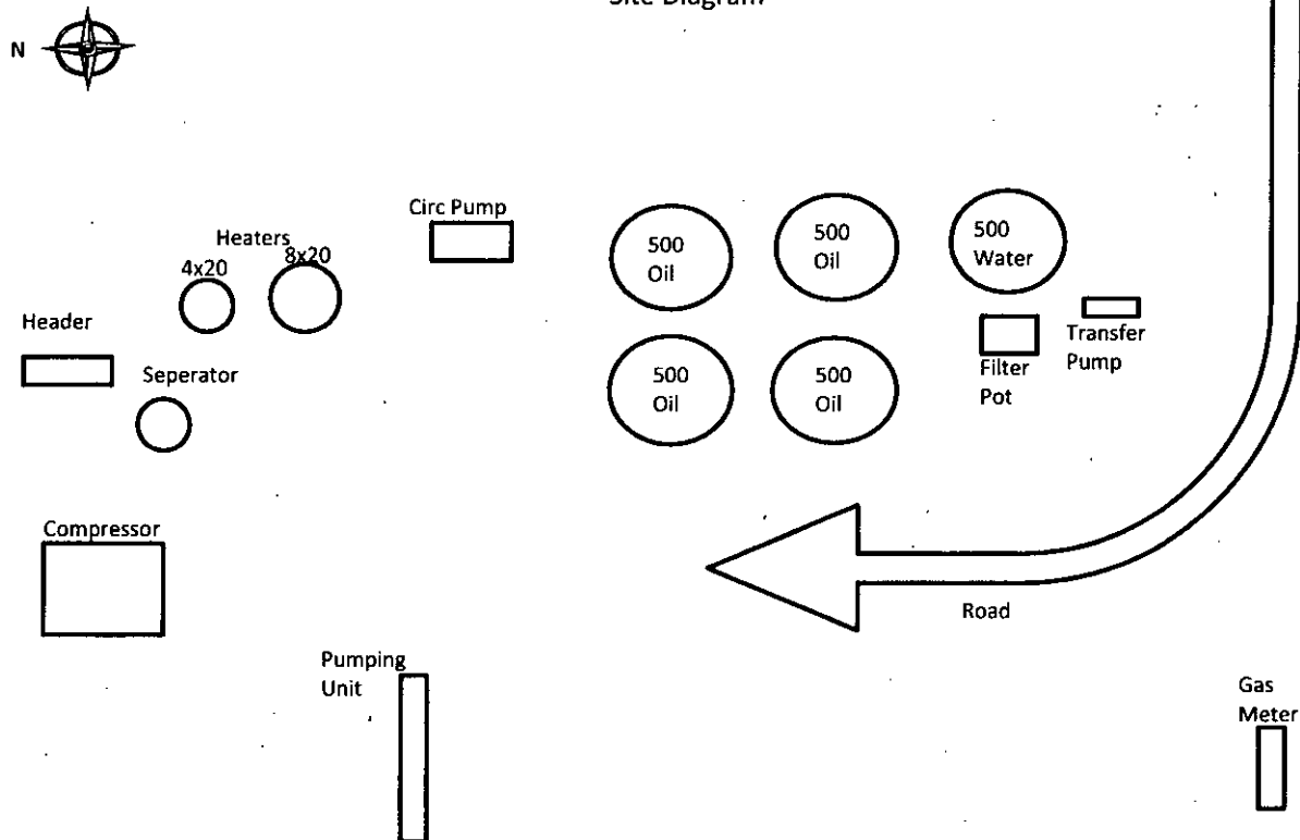
Site Diagram
