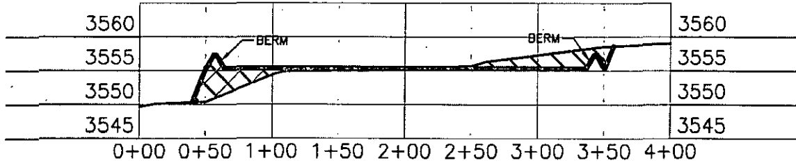
SECTION C-C'
