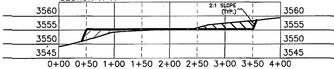
SECTION B-B'
