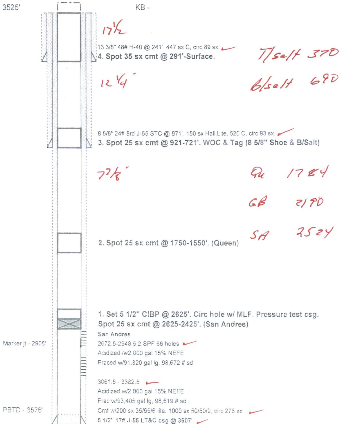
RJ Unit #136 Wellbore diagram
