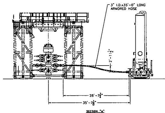
SECTION "A"
