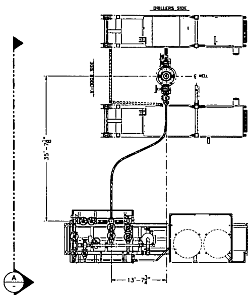
PLAN VIEW
