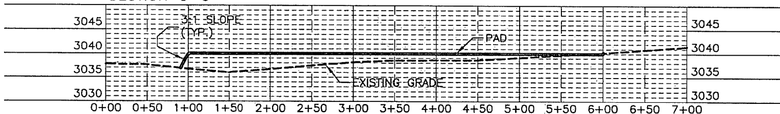
SECTION C-C'
