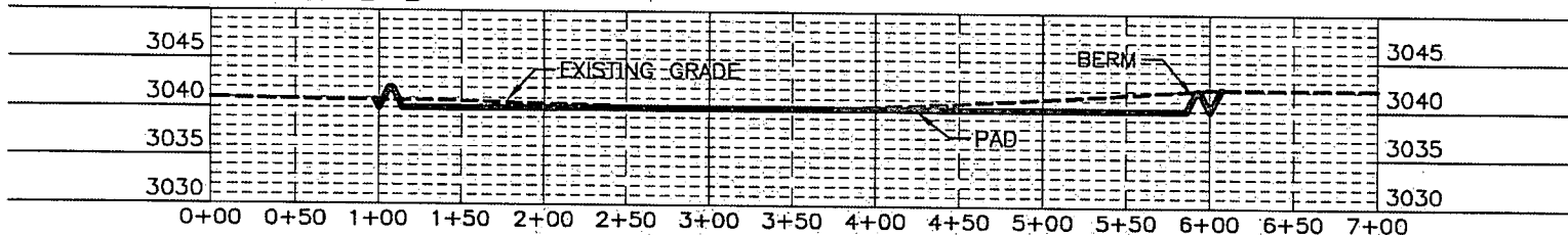
SECTION B-B'
