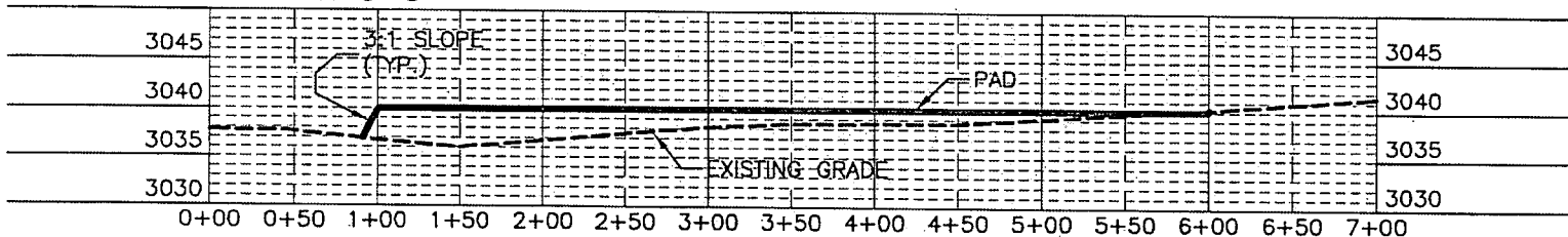
SECTION C-C'
