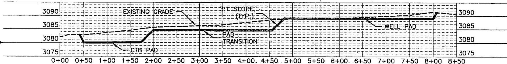
SECTION E-E'
