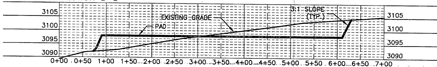
SECTION B-B'
