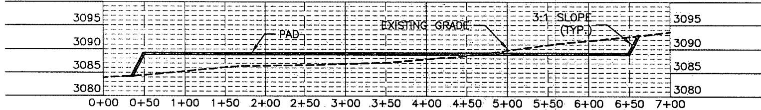
SECTION D-D'
