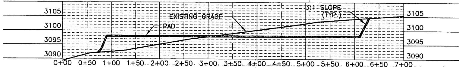
SECTION B-B'
