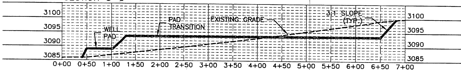
SECTION C-C'
