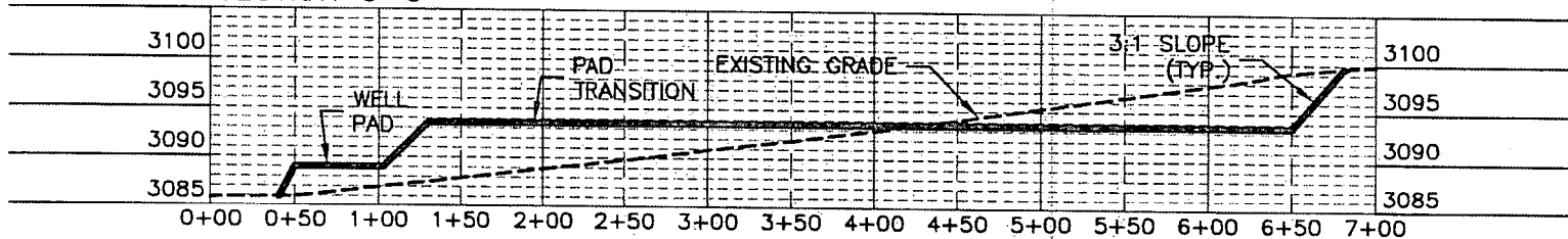
SECTION C-C'
