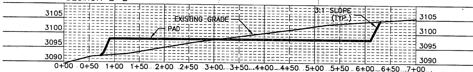
SECTION B-B'
