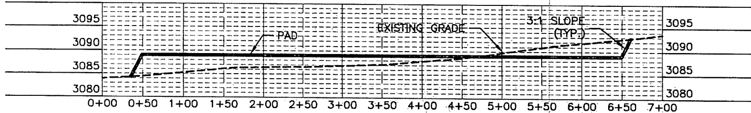
SECTION D-D'
