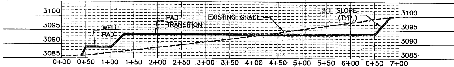
SECTION C-C'
