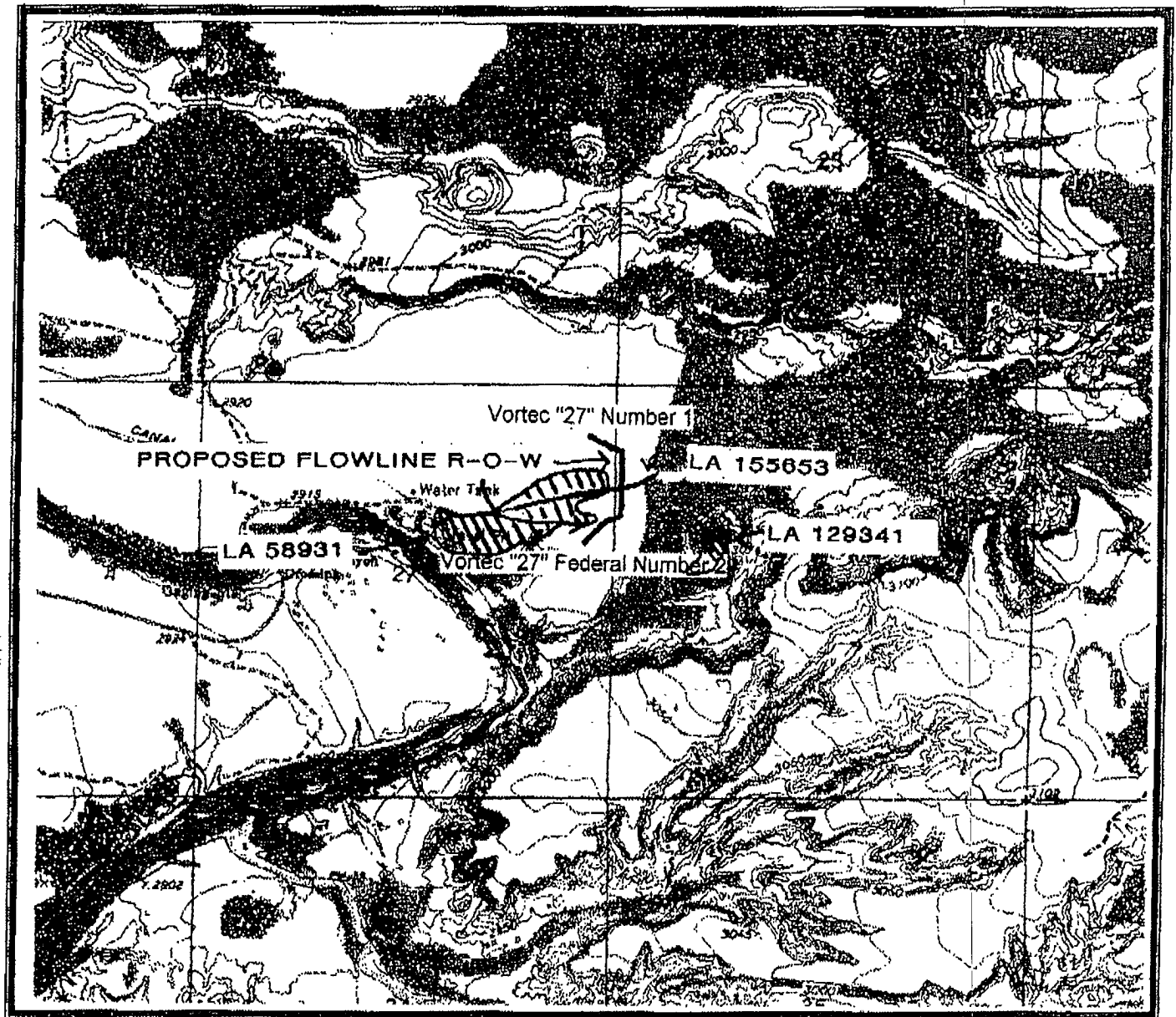
Figure 1: Survey Area Pogo Producing Company The Proposed Flowline Right-of-Way from the Vortec "27" Federal Number 2 to the Vortec "27" Number 1 Well Locations, and Site LA 155,653 Sections 26 and 27, T. 24S, R.30E USGS Pierce Canyon, NM (1968) 7.5' topo map Eddy County, New Mexico Scale 1:24,000
