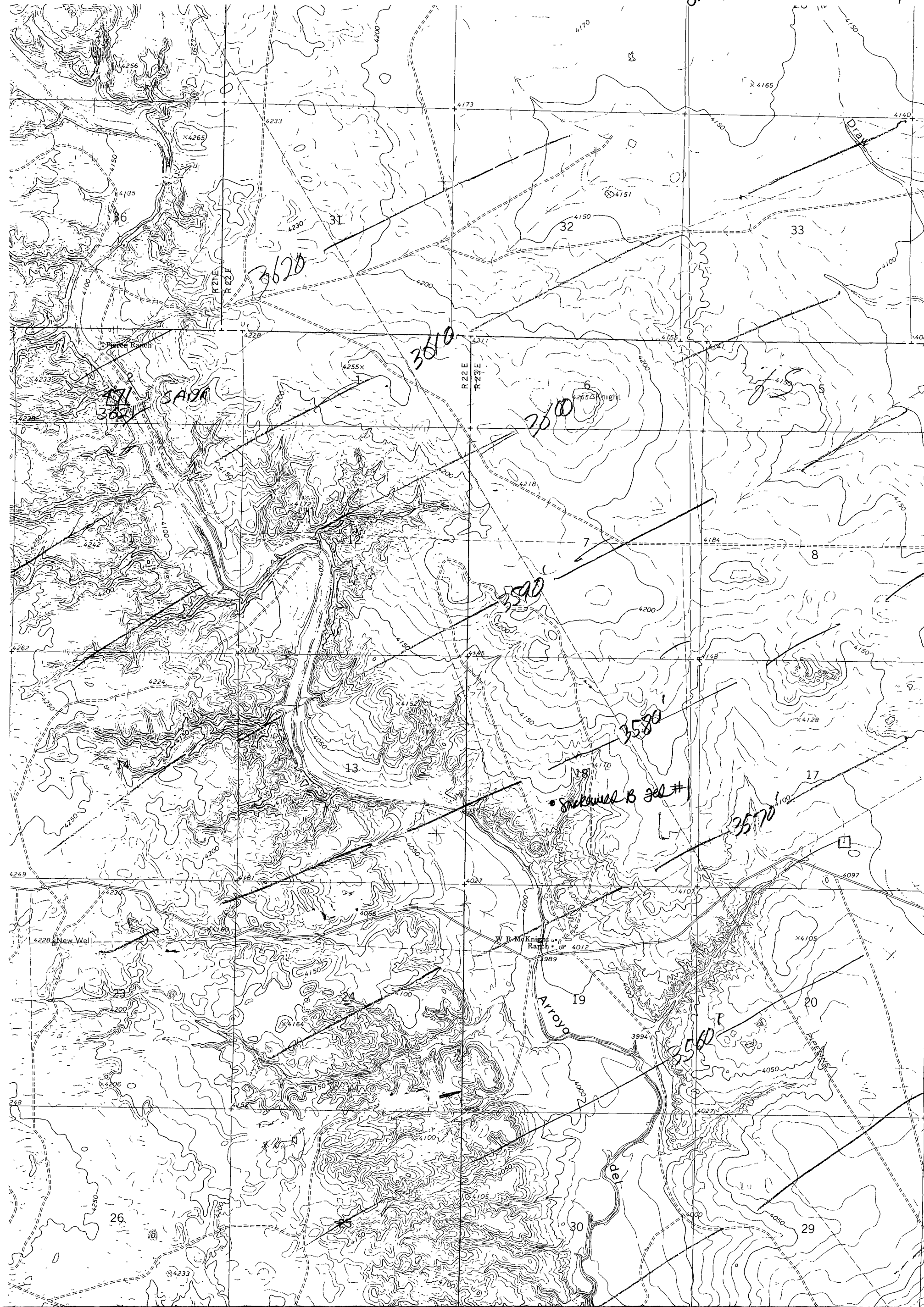
Groundwater table map of San Andres Aquifer interpretation based on New Mexico State Engineer data.
