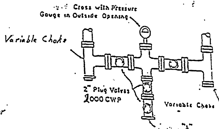
PLAN VIEW-CHOKER MANIFOLD
