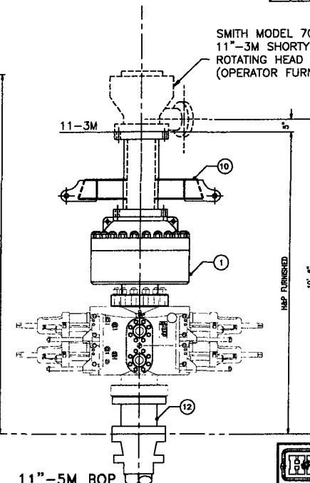
11"-5M BOP W/ ROTATING HEAD
