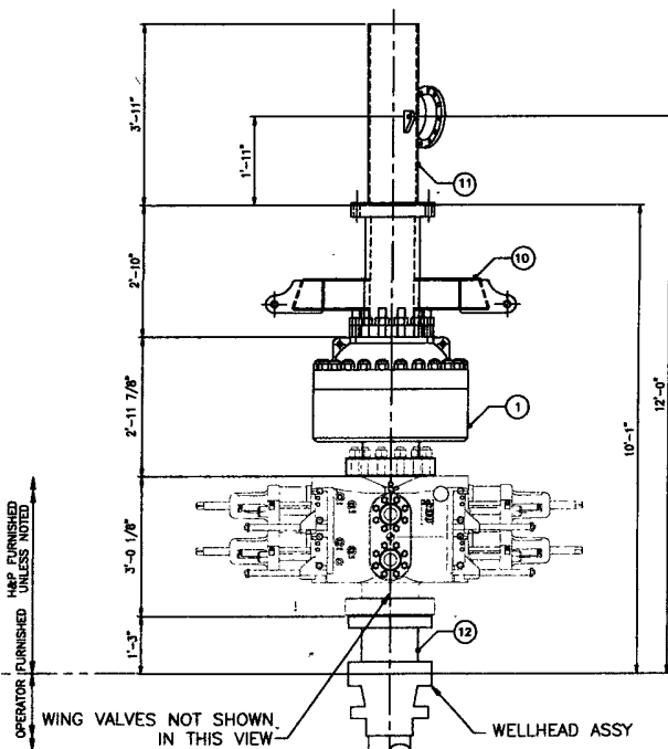
11"-5M BOP W/ BELL NIPPLE
