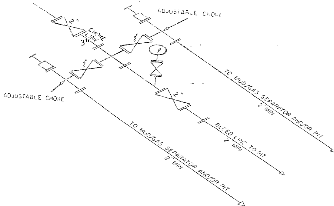
2M CHOKE MANIFOLD EQUIPMENT — CONFIGURATION OF CHOKES 0 MAY VARY
