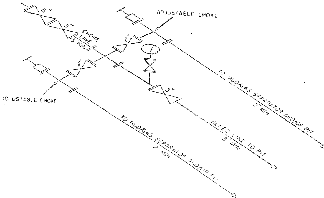
3M CHOKER MANIFOLD EQUIPMENT — CONFIGURATION OF CHOKES MAY VARY
