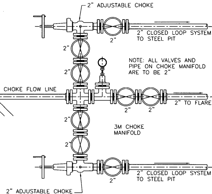
CHOKE MANIFOLD PLAN
