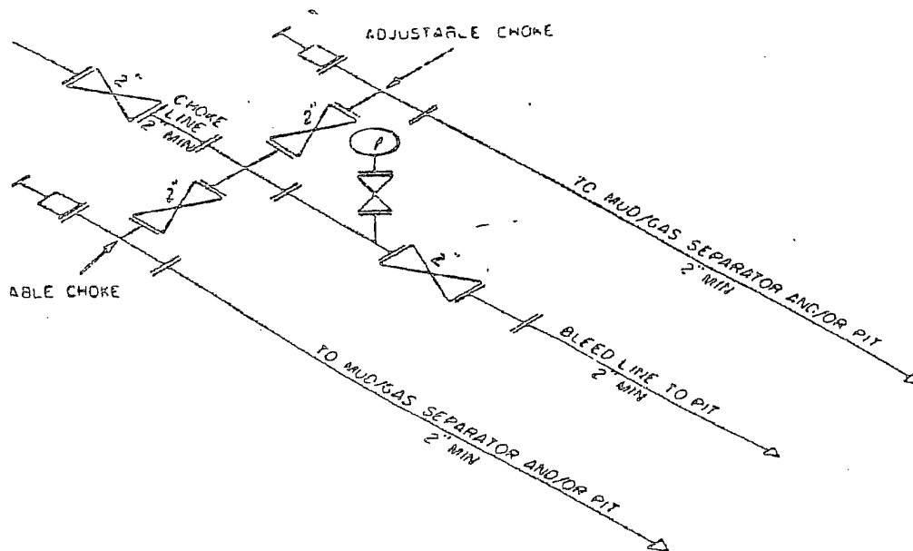
2M CHOKE MANIFOLD EQUIPMENT — CONFIGURATION OF CHOKES
