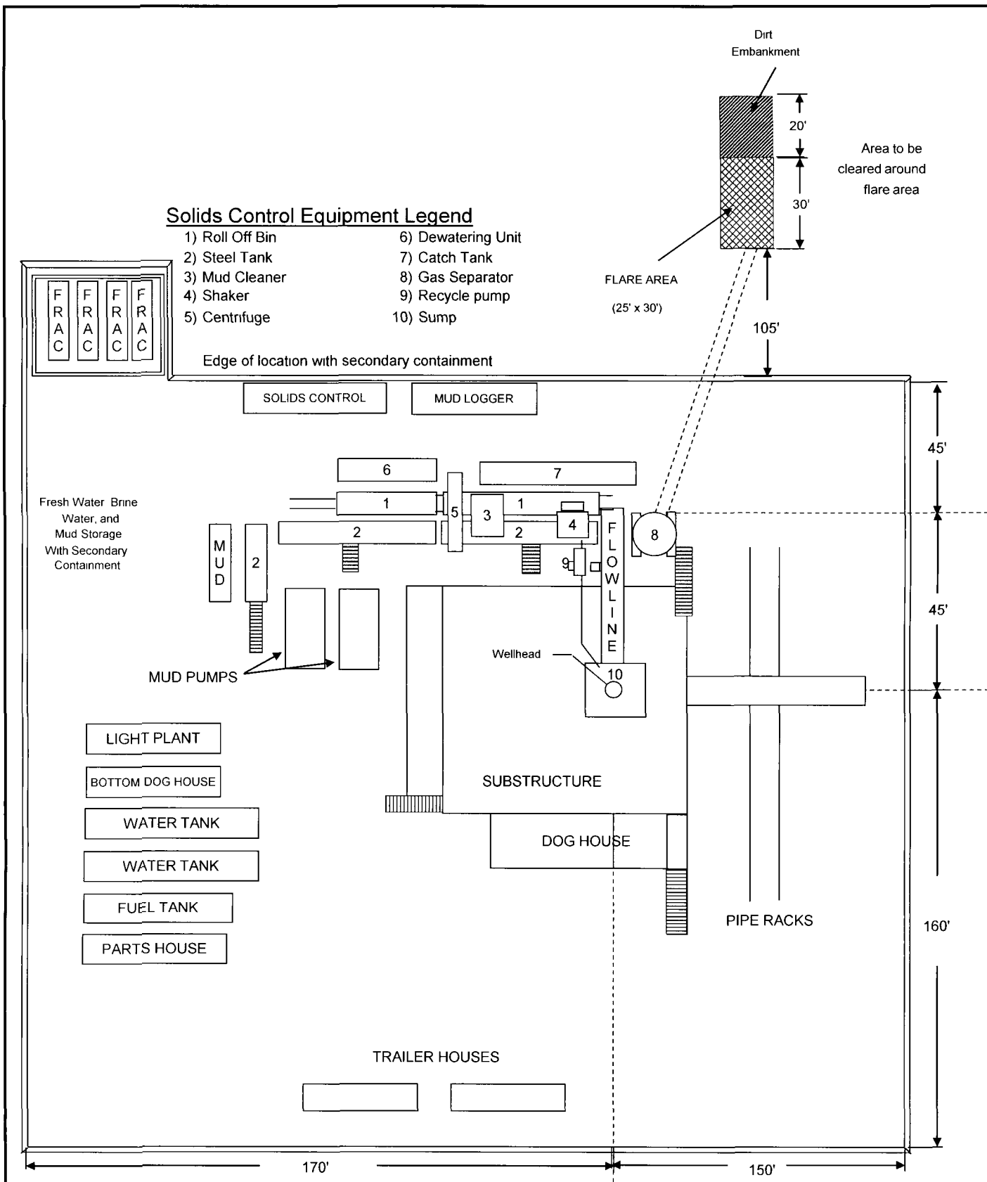
POKER LAKE UNIT 341H TYPICAL RIG LAYOUT SCHEMATIC INCLUSIVE OF CLOSED-LOOP DESIGN PLAN
