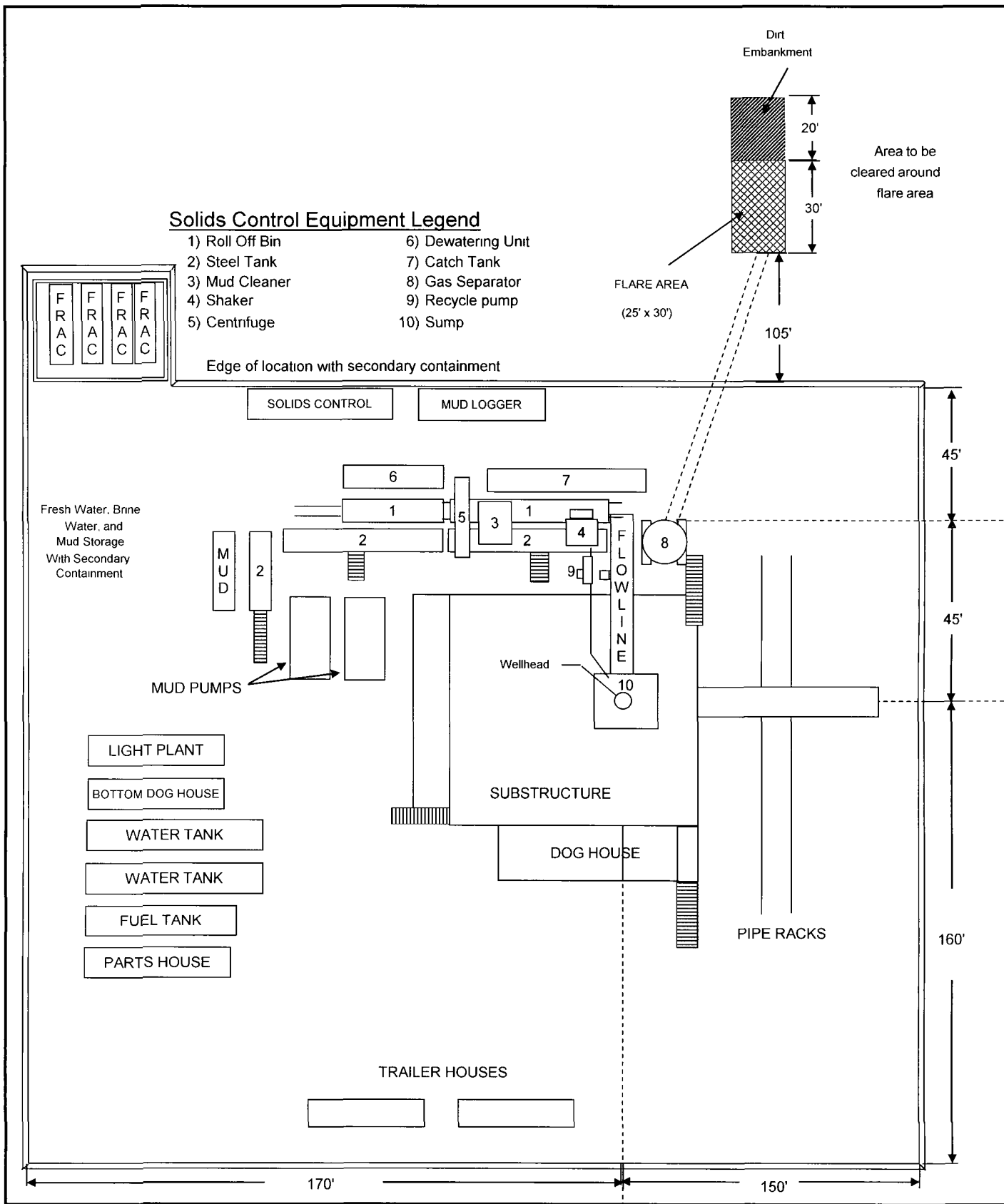
POKER LAKE UNIT 345H TYPICAL RIG LAYOUT SCHEMATIC INCLUSIVE OF CLOSED-LOOP DESIGN PLAN
