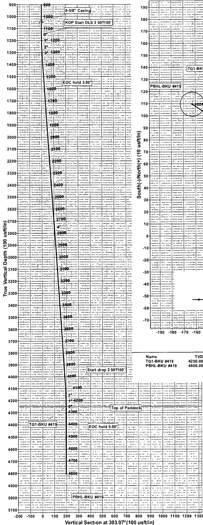
PROJECT DETAILS: Eddy County, NM (NAN27 NME) Plan Plan #2 8-3/4" Hole (Burch Keely Unit #419/OH)
