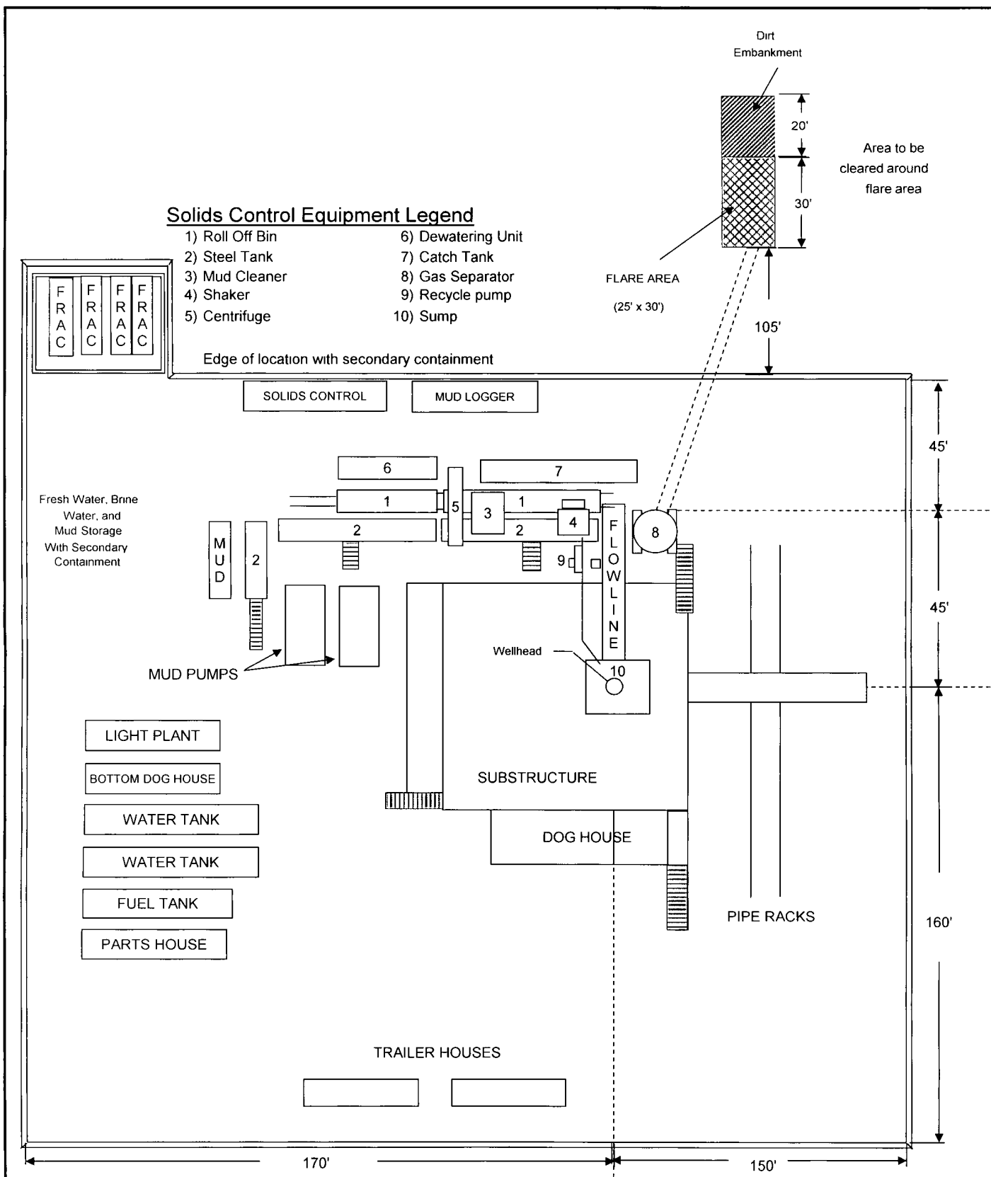
POKER LAKE UNIT 368H TYPICAL RIG LAYOUT SCHEMATIC INCLUSIVE OF CLOSED-LOOP DESIGN PLAN
