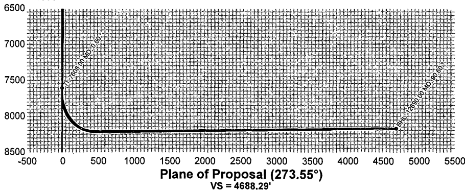
Vertical Section Plot 1" = 1000'
