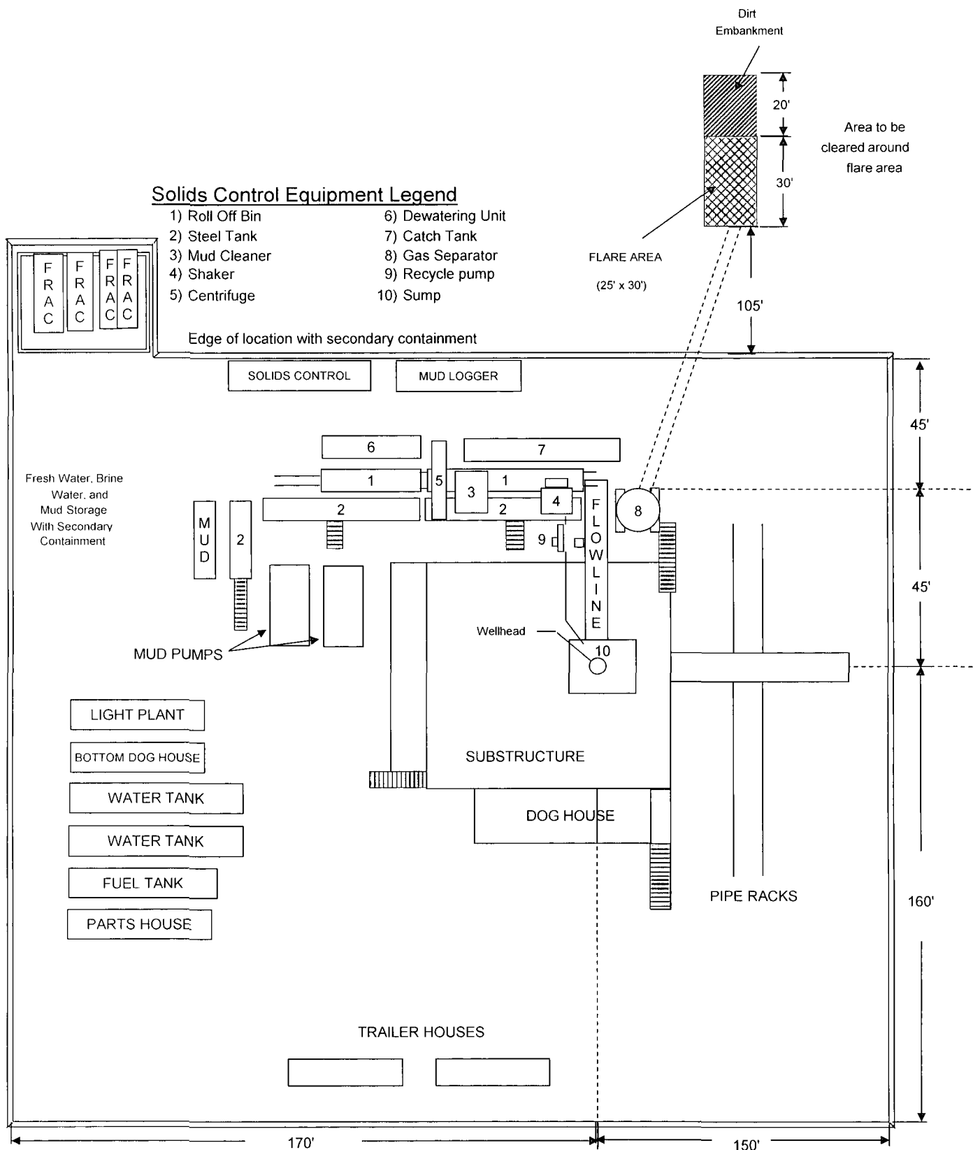
BIG EDDY UNIT 256H TYPICAL RIG LAYOUT SCHEMATIC INCLUSIVE OF CLOSED-LOOP DESIGN PLAN
