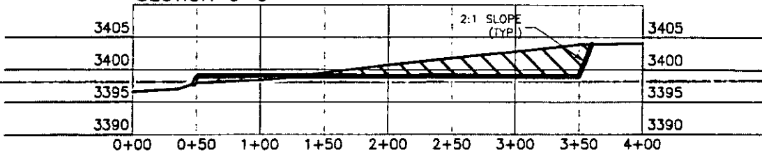
SECTION C-C'
