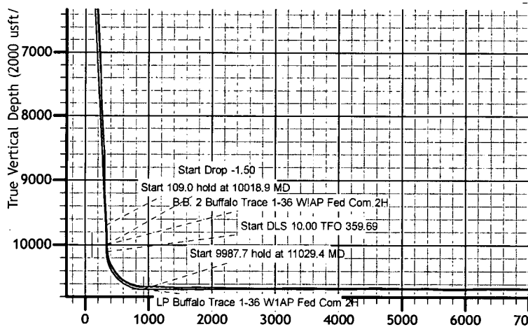
Vertical Section at 1.64° (2000 usft/in)
