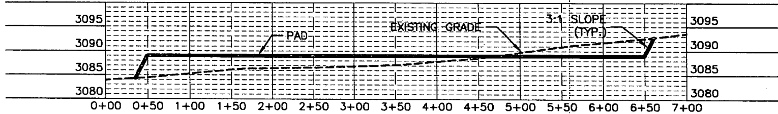
SECTION D-D'
