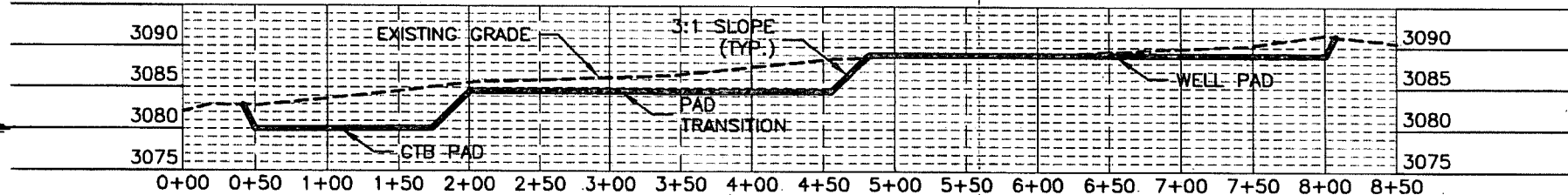
SECTION E-E'
