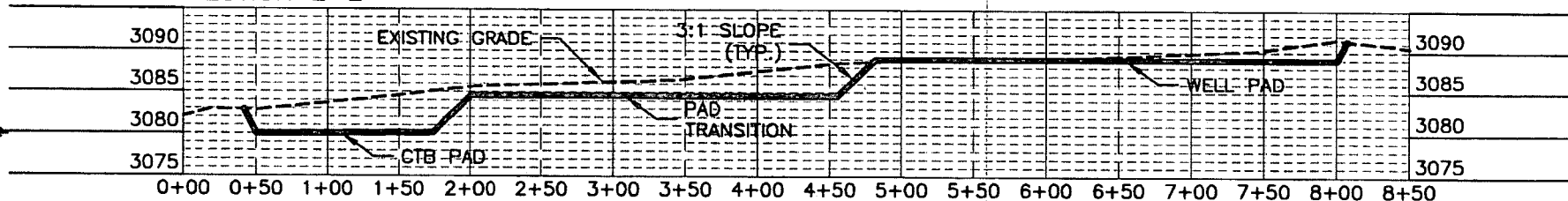
SECTION E-E'
