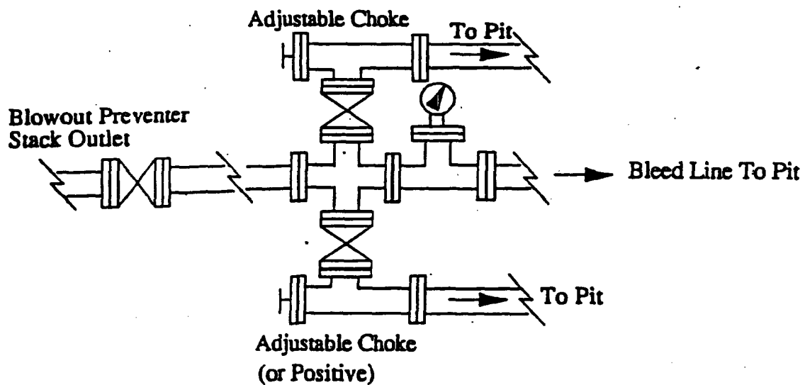
Choke Manifold
